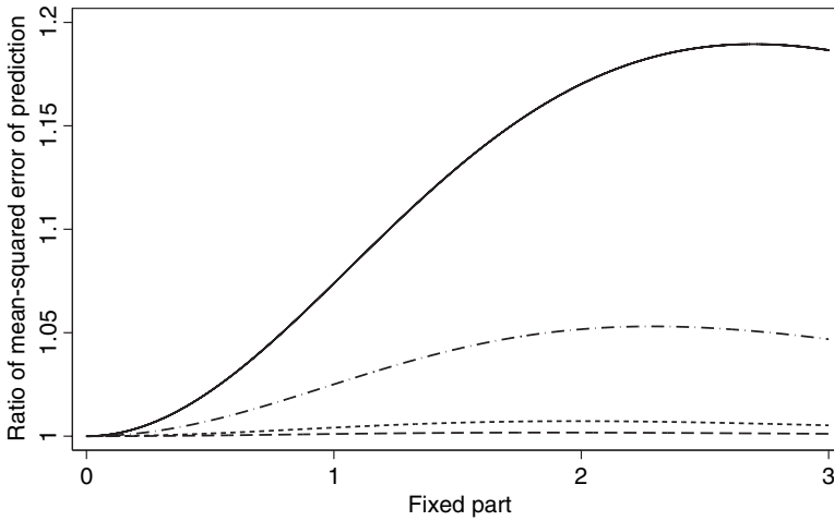
Fig. 5. Ratio of the MSEP comparing the median with population-averaged response probabilities for four values of the intraclass correlation of the latent responses when the fixed part \mathbf{x}^0\beta ranges from 0 to 3 with ICC^* = 0.1 (---), ICC^* = 0.2 (-·-·-·-), ICC^* = 0.5 (·-·-·-·) and ICC^* = 0.8 (—)
